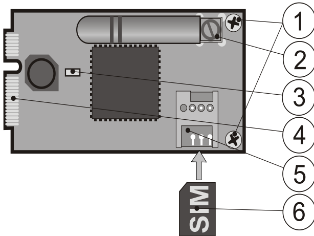
Afb. 1 :De JA-194Y communicator
